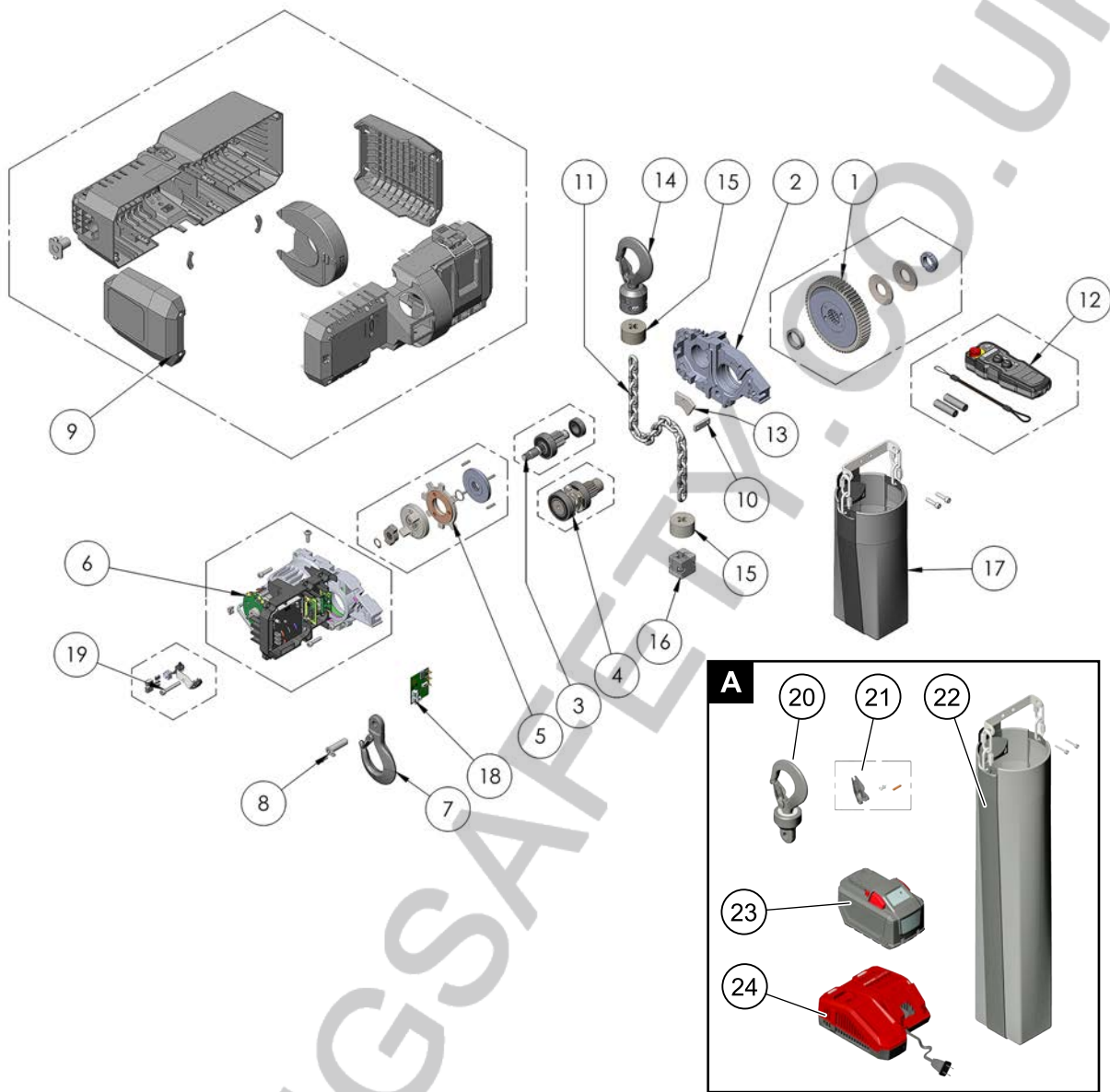
Figure 14. Hoist Parts
