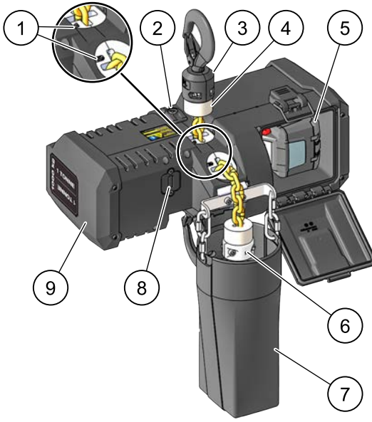
Figure 2. Hoist Features
