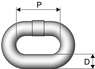
Figure 8. Chain Dimensions
