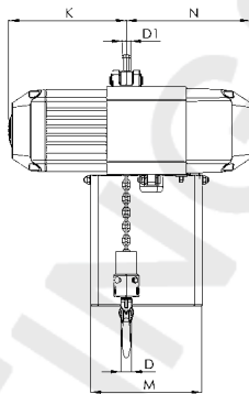
Model CPV/CPVF with suspension lug, 250 - 2500 kg, single fall
