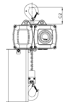
Model CPV/CPVF with suspension hook, 250 - 2500 kg
