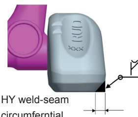
Picture 3: HY-weld seam
