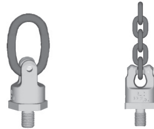
lifting points for bolting PP-S / PP-B / PP-VIP
