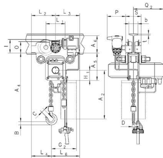
Model CPA with integrated pneumatic trolley
