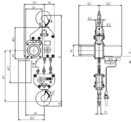
Model CPA with suspension hook, 7500 kg, three fall
