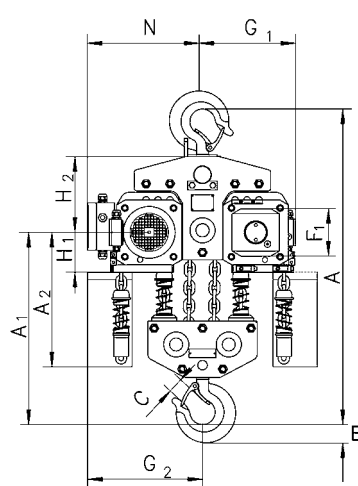
Model CPE/CPEF 100-2 with suspension hook, 10000 kg
