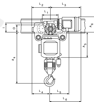
Model CPE/CPEF with integrated electric trolley
