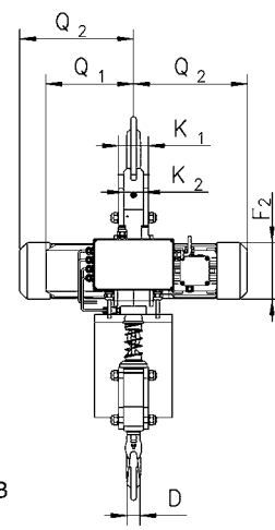
Model CPE/CPEF 100-2 with suspension hook, 10000 kg
