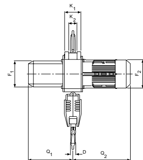
Model CPE/CPEF with suspension hook, 3200 - 5000 kg, double fall
