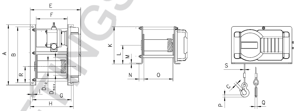
Rope lead-offs for electric rope winch RPE
