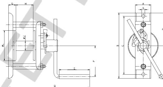
Model MWS with spur gear drive Capacity 125 kg
