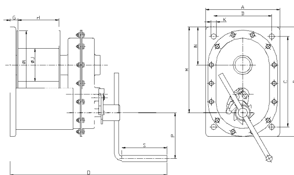
Model MWS with spur gear drive Capacities 1.000 - 2.000 kg
