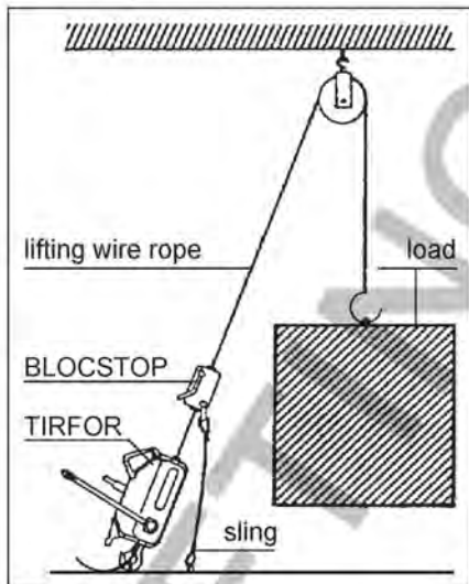
Fig. 4 - BLOCSTOP on lifting wire rope
