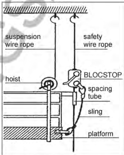
Fig. 5 - BLOCSTOP on safety wire rope
