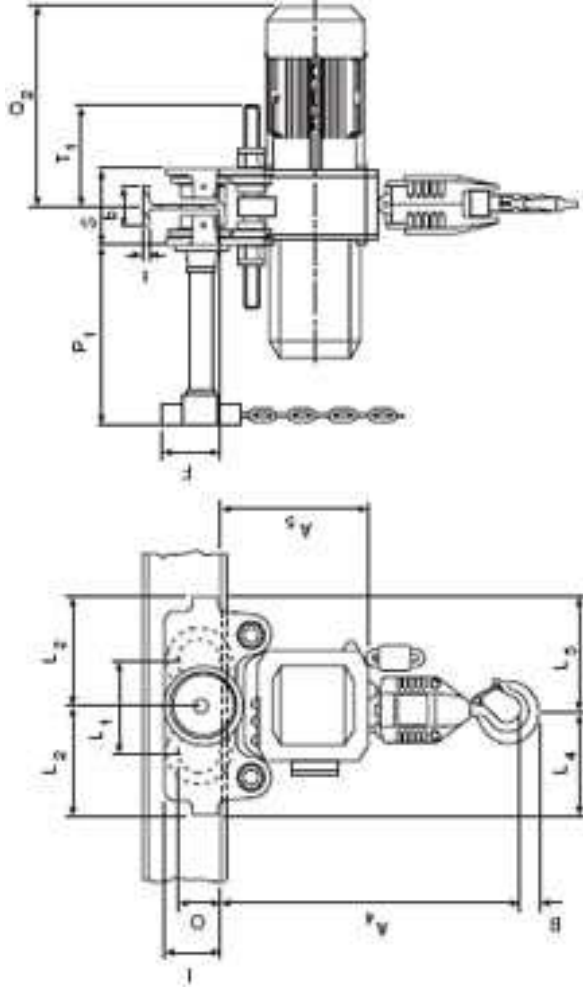
Model CPE with integral push or geared trolley
