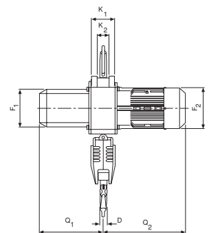
Model CPE with suspension hook, double fall 3.200 - 5.000 kg
