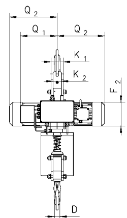
Model CPE 100-2 with suspension hook 10.000 kg
