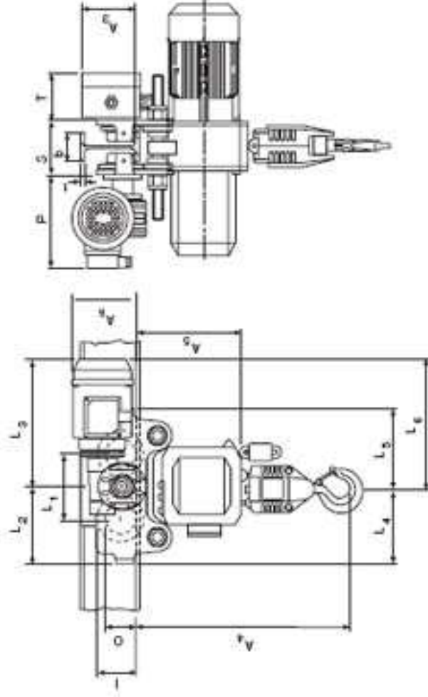
Model CPE with integral electric trolley
